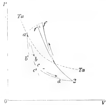
FIG. 6.—Adiabatics.
